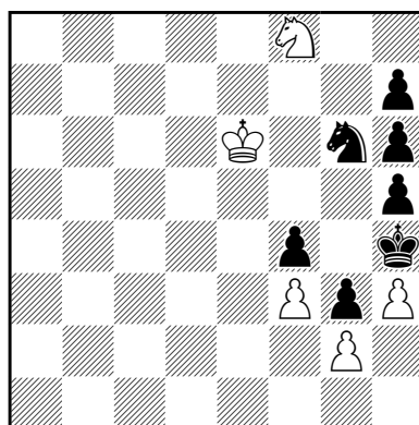
458 h#3* (5+7)
