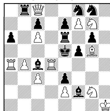
489 #3 (12+13)
