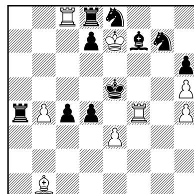
507 #9 (8+10)
