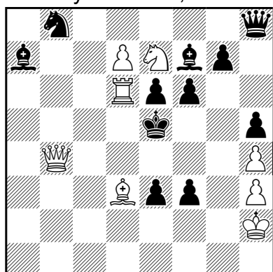
505 #4 (8+11)
