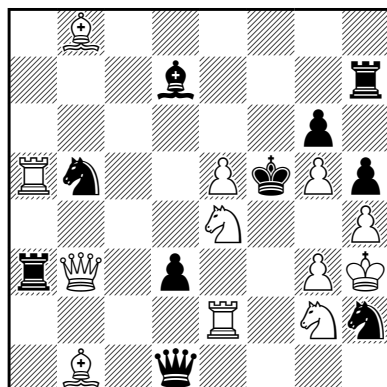
412 #2 (12+10)
