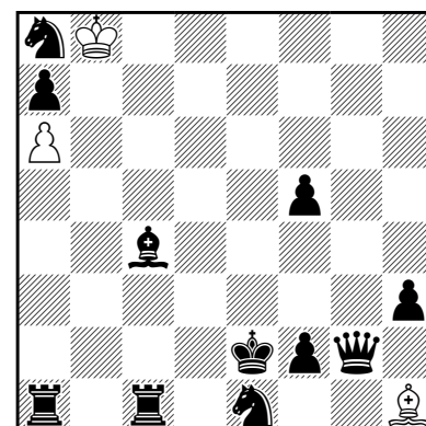
462 h#4 (3+11)
