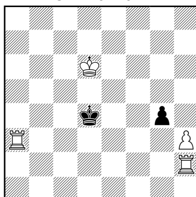
485 #3 (4+2)
