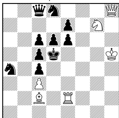
502 #2 (6+10)
