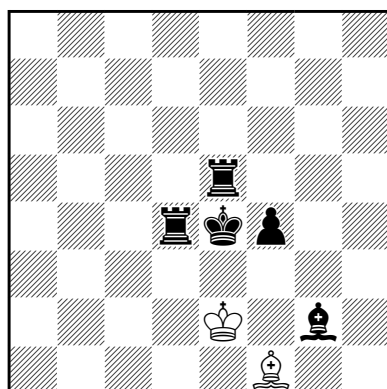
467 h#4 (2+5)
