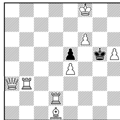
416 #2 (8+2)
