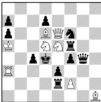
415 #2 (8+11)
