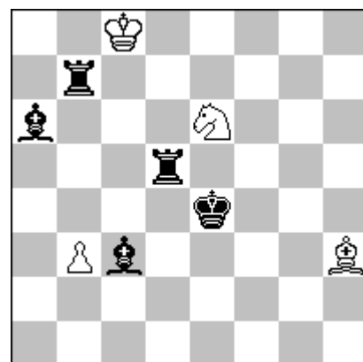
h # 3 b)b3→b4 (4 + 5)
