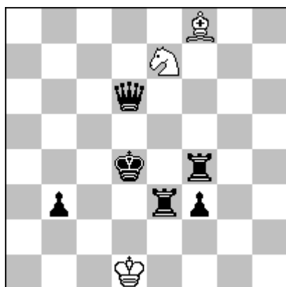
h # 3 b)f3→d3 (3 + 6)
