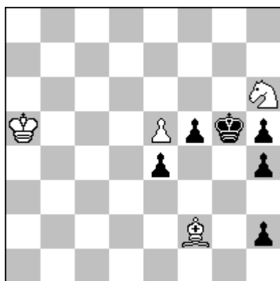
h # 3 b)f5→g2 (4 + 6)
