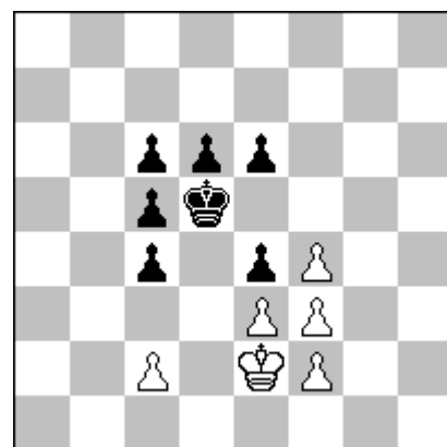
h # 3 b)e6→e5 (6 + 7)
